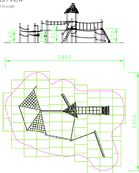
Plan View Not to scale
